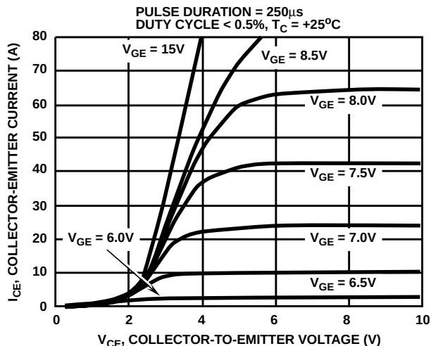
FIGURE 2. SATURATION CHARACTERISTICS (TYPICAL)
