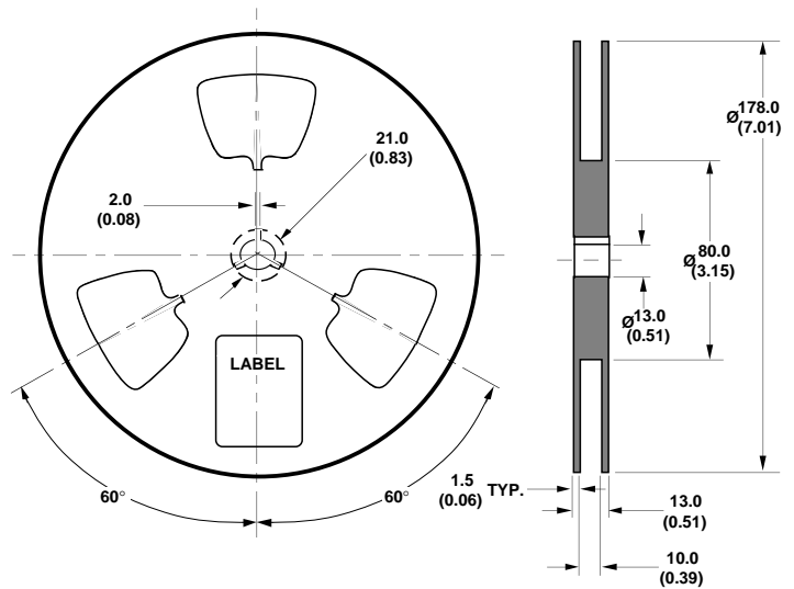
Figure 9. Reel Dimensions.
