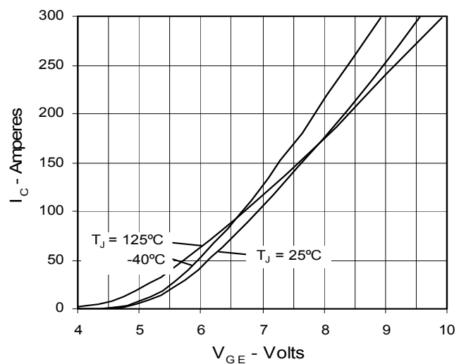
Fig. 6. Input Admittance
