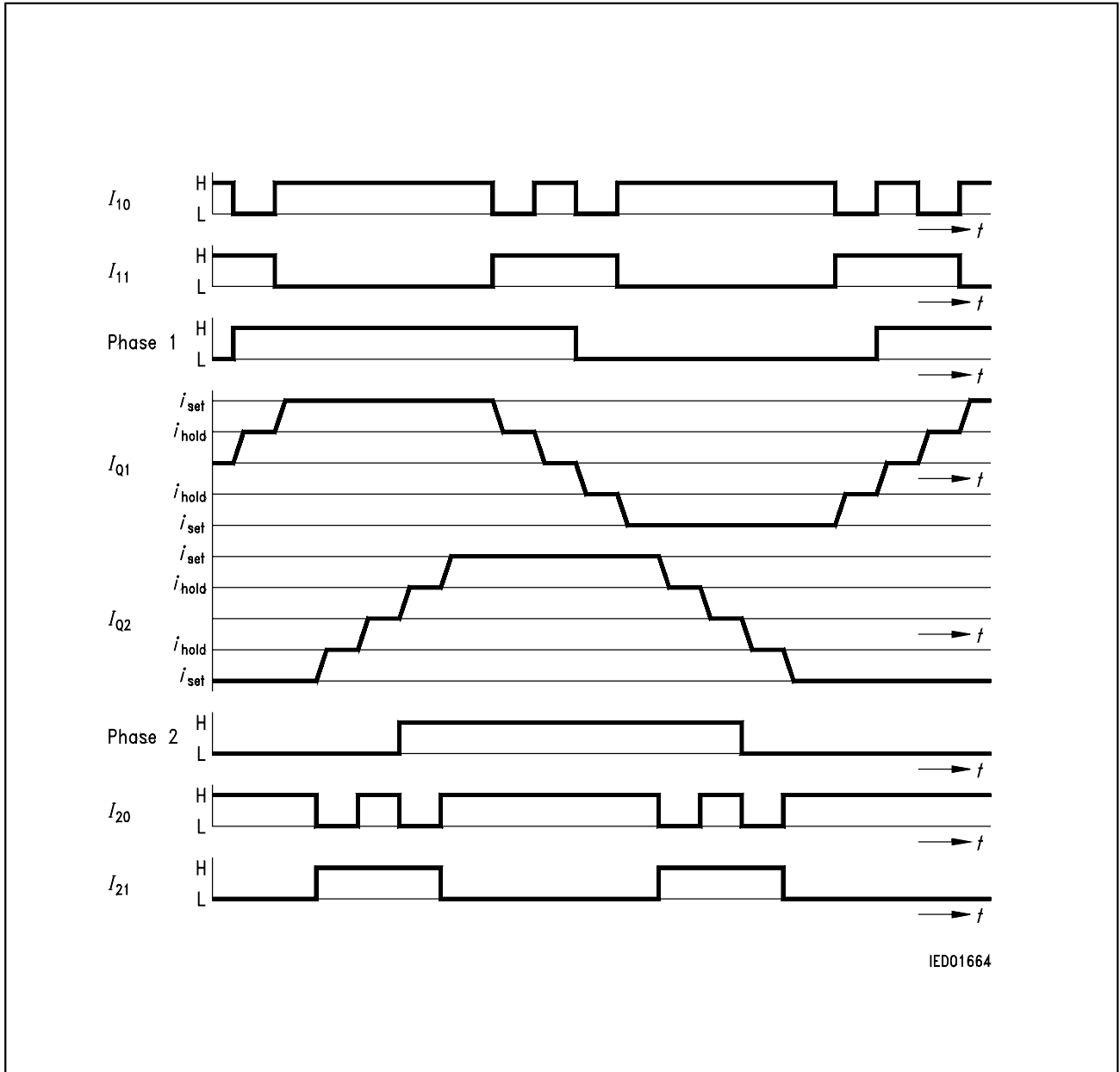
Figure 8 Quarter-Step Operation
