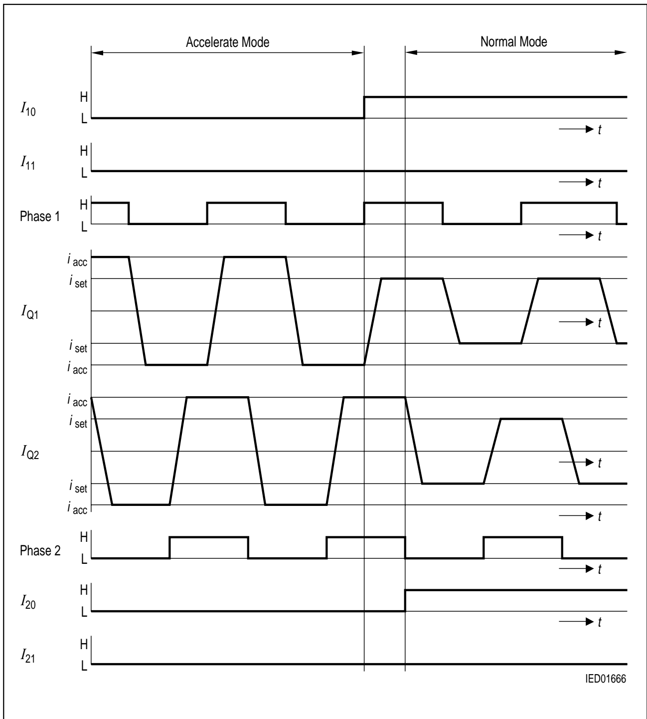
Figure 6 Full-Step Operation
