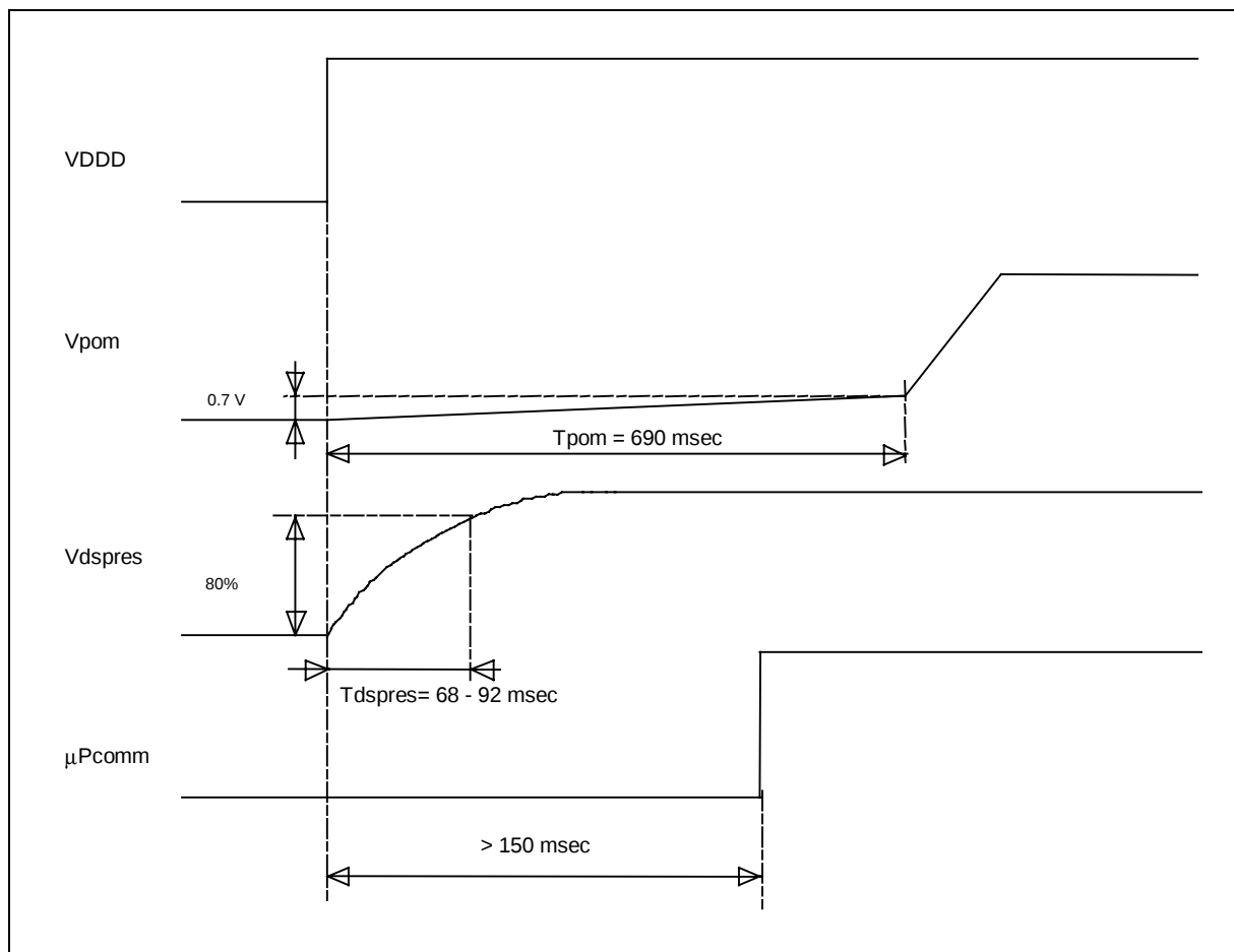
Fig. 8.6 Power-up timing diagram to avoid clicks
