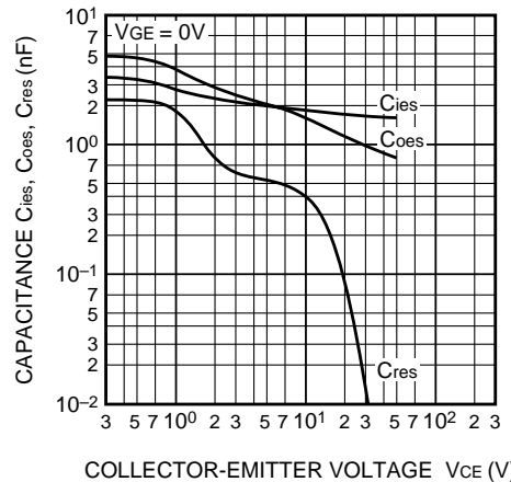
CAPACITANCE VS. Vce (TYPICAL)
