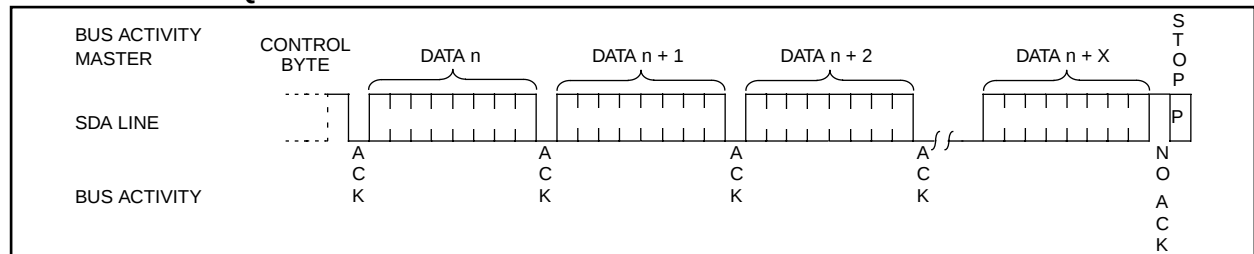
FIGURE 8-3: SEQUENTIAL READ
