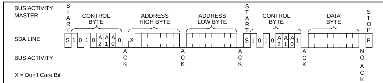
FIGURE 8-2: RANDOM READ
