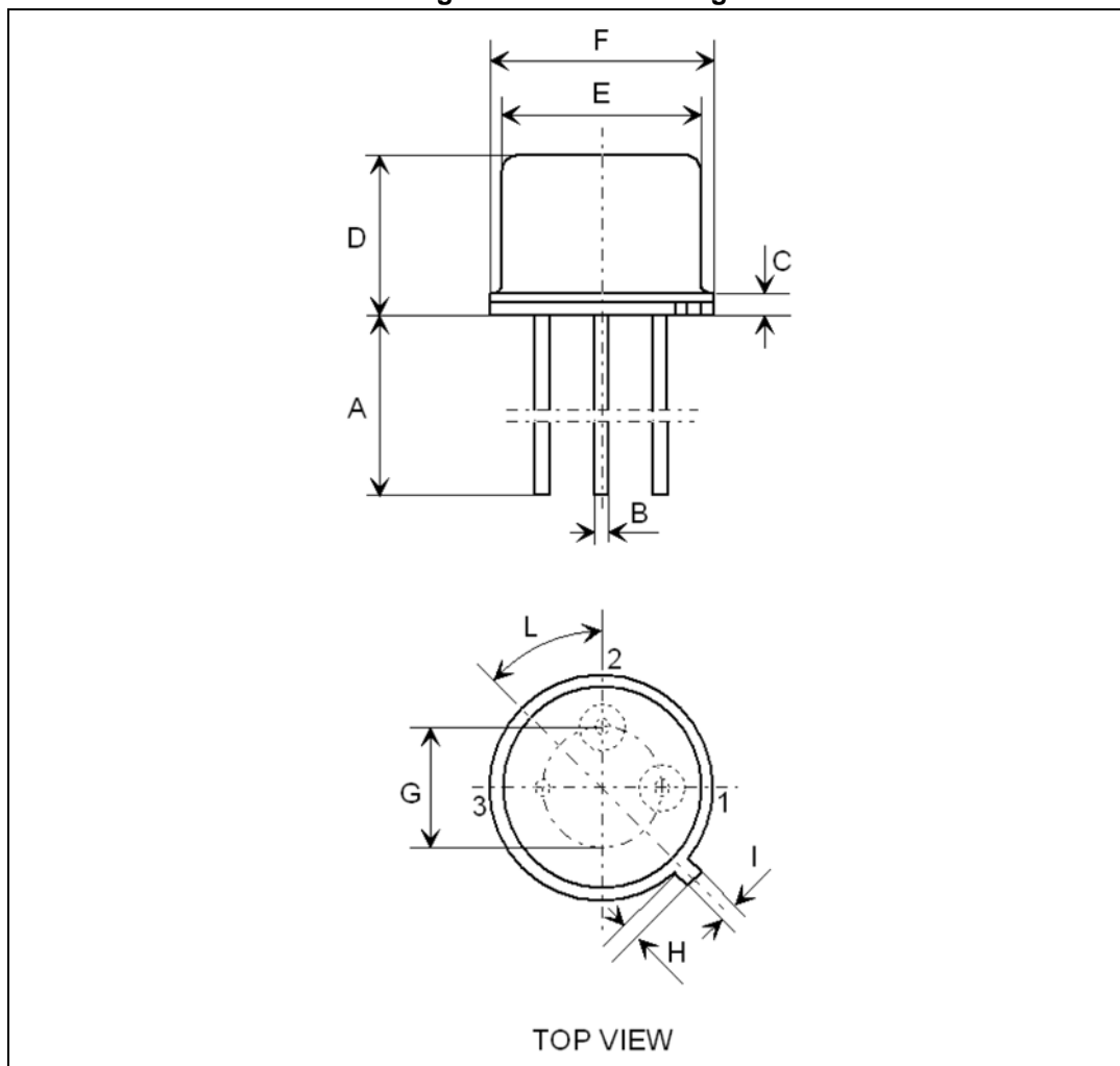
Figure 9. TO-39 drawing
