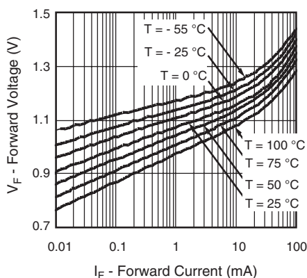
Fig. 3 - Diode Forward Voltage vs. Forward Current
