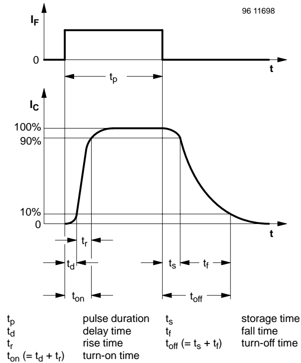
Figure 2. Switching times
