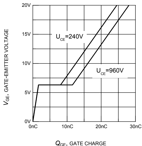
Figure 18. Typical gate charge ( I_C = 3A )
