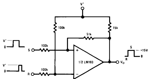
Bi-Stable Multivibrator
