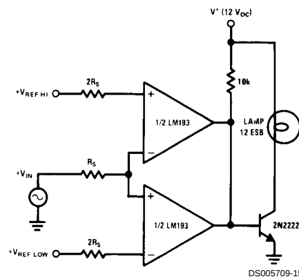
Limit Comparator
