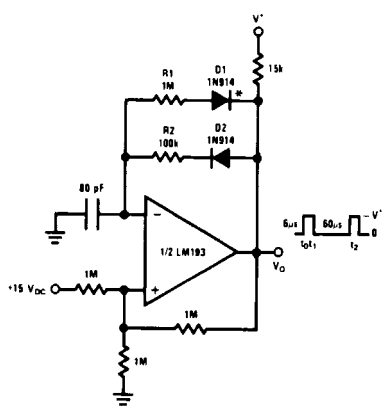
Pulse Generator
