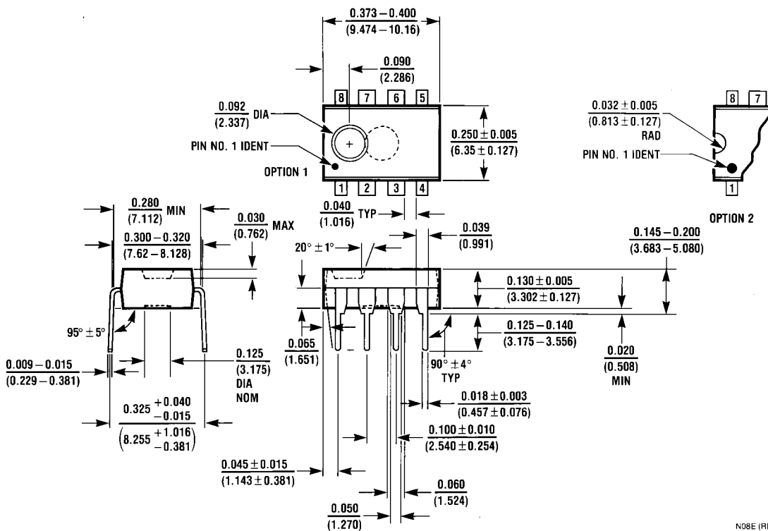
Molded Dual-In-Line Package (N) Order Numbers LM393N or LM2903N NS Package Number N08E
