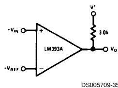
Basic Comparator
