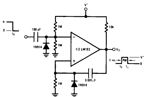
One-Shot Multivibrator
