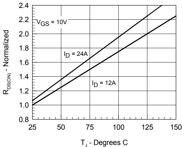
Fig.5 Temperature Dependence of Drain-to-Source Resistance
