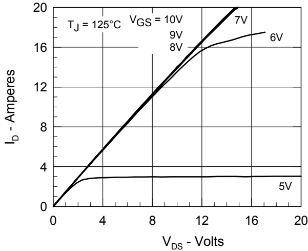
Fig.3 Output Characteristics @ T_J = 125^\circ\text{C}
