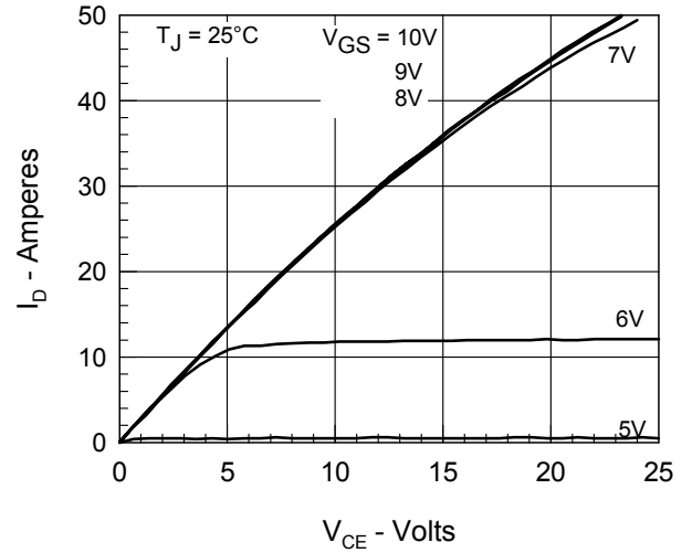
Fig.2 Extended Output Characteristics @ T_J = 25^\circ\text{C}
