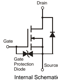
Internal Schematic
