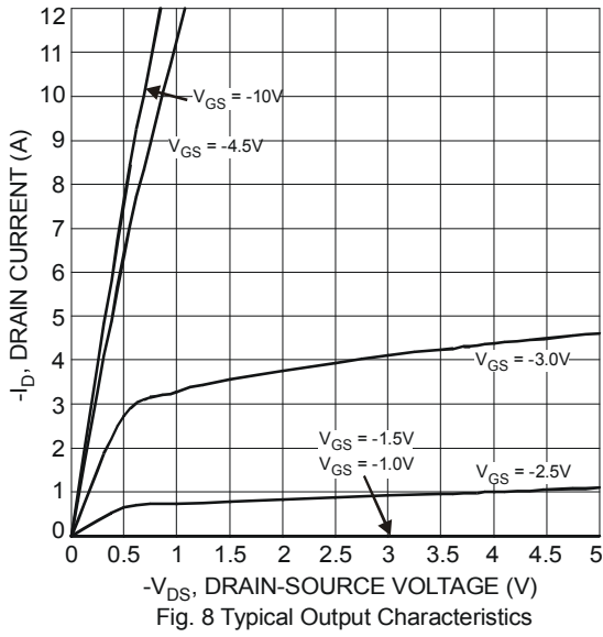
Fig. 8 Typical Output Characteristics
