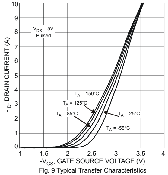
Fig. 9 Typical Transfer Characteristics
