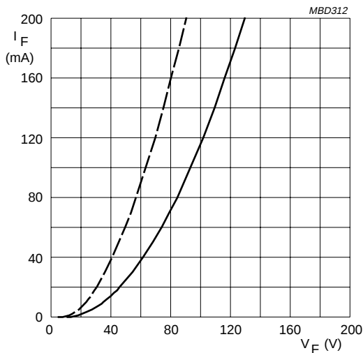
BY8016. Dotted line: T_j = 120^\circ\text{C} . Solid line: T_j = 25^\circ\text{C} .
