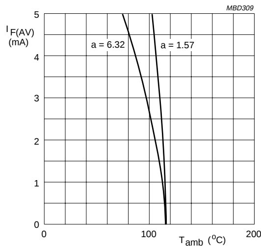
BY8012. a = I_{F(RMS)}/I_{F(AV)} ; V_R = V_{RWmax} ; R_{th\ j-a} \leq 120 K/W. a = 1.57 : half sinewave. a = 6.32 : line output transformer application; see see Fig.18.
