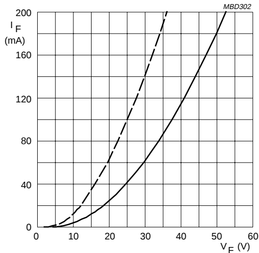
BY8006. Dotted line: T_j = 120^\circ\text{C} . Solid line: T_j = 25^\circ\text{C} .
