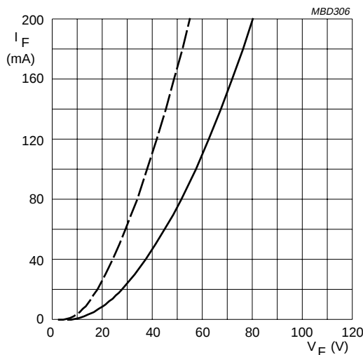
BY8010. Dotted line: T_j = 120^\circ\text{C} . Solid line: T_j = 25^\circ\text{C} .
