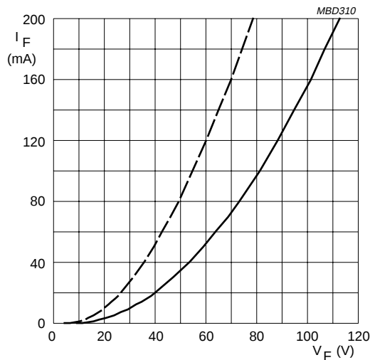
BY8014. Dotted line: T_j = 120^\circ\text{C} . Solid line: T_j = 25^\circ\text{C} .
