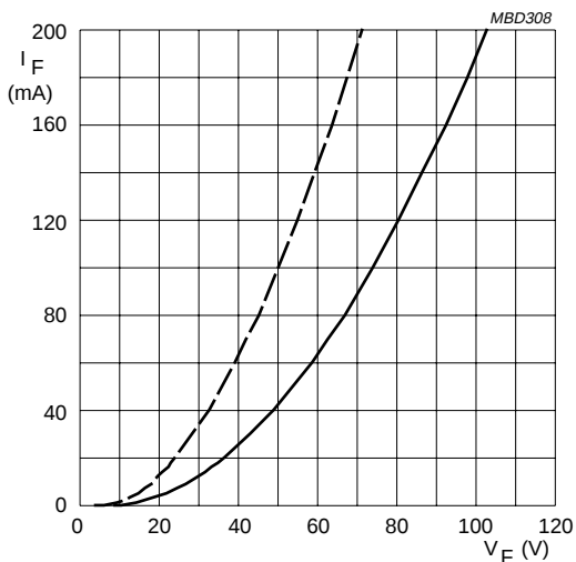
BY8012. Dotted line: T_j = 120^\circ\text{C} . Solid line: T_j = 25^\circ\text{C} .
