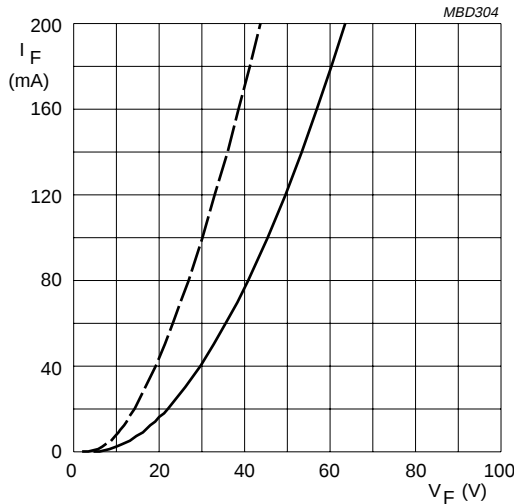
BY8008. Dotted line: T_j = 120^\circ\text{C} . Solid line: T_j = 25^\circ\text{C} .
