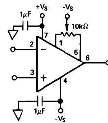
Figure 20. Standard Null Circuit
