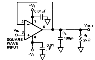
Figure 21c. Unity Gain Follower-AD542/AD547
