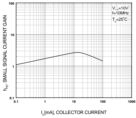
Figure 7. High Frequency Current Gain
