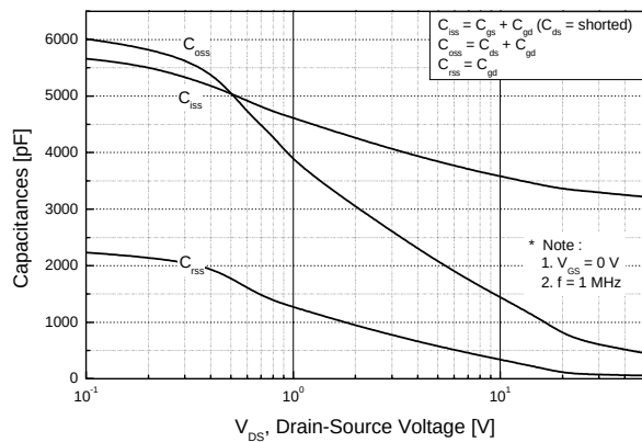
Figure 5. Capacitance Characteristics
