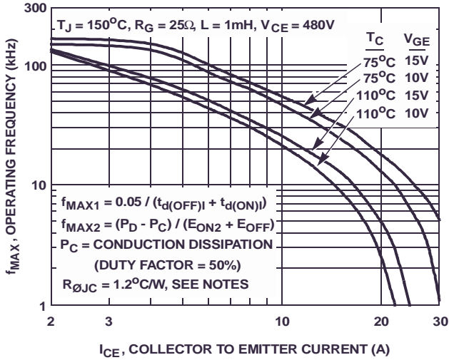
FIGURE 3. OPERATING FREQUENCY vs COLLECTOR TO EMITTER CURRENT
