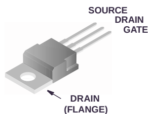
HUFA76439P3
