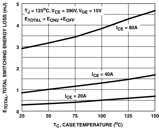
FIGURE 15. TOTAL SWITCHING LOSS vs CASE TEMPERATURE
