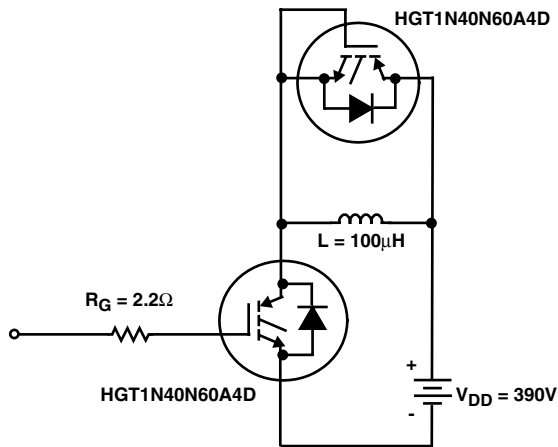
FIGURE 24. INDUCTIVE SWITCHING TEST CIRCUIT
