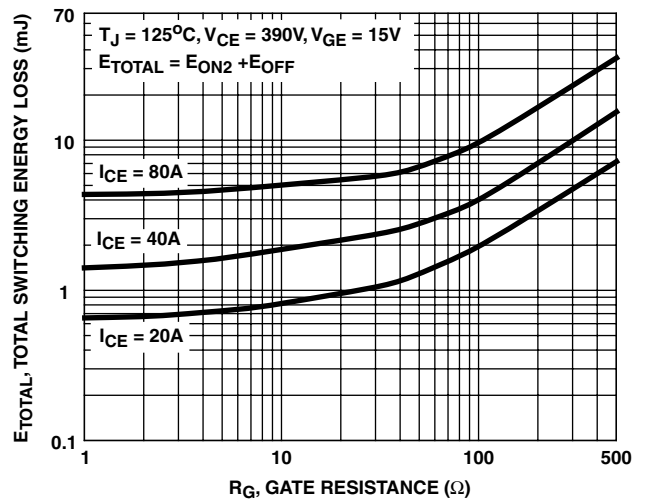
FIGURE 16. TOTAL SWITCHING LOSS vs GATE RESISTANCE
