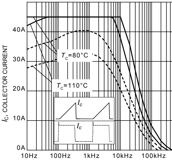
Figure 1. Collector current as a function of switching frequency ( T_j \leq 150^\circ\text{C} , D = 0.5 , V_{CE} = 600\text{V} , V_{GE} = 0/+15\text{V} , R_G = 56\Omega )
