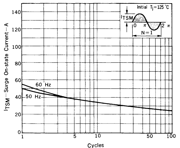
Fig. 2 I_{TSM} RATING
