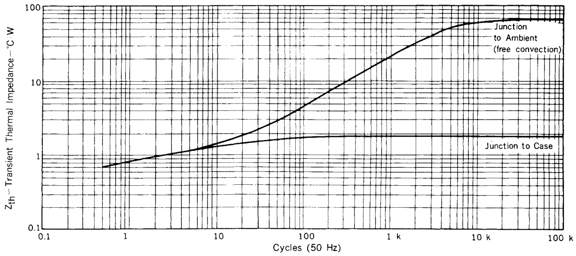
Fig. 13 Z_{th} CHARACTERISTIC
