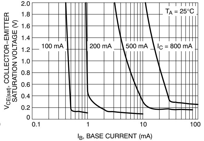
Figure 4. Saturation Region
