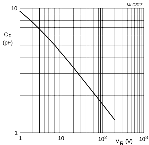
BYD43-16 to 20 f = 1 \text{ MHz}; T_j = 25 \text{ }^\circ\text{C}.
