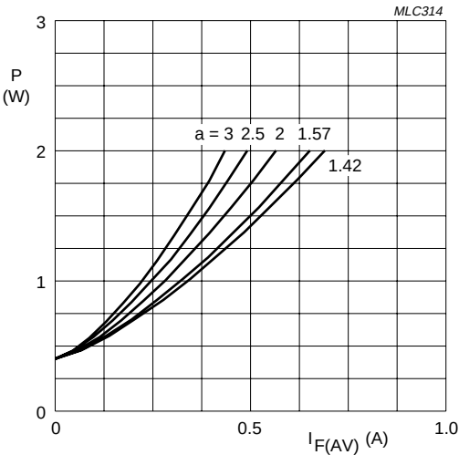
BYD43-16 to 20 a = I_{F(RMS)}/I_{F(AV)} ; V_R = V_{RRMmax} ; \delta = 0.5 .
