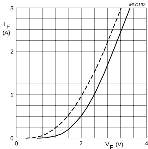
BYD43-16 to 20 Dotted line: T_j = 175\text{ }^{\circ}\text{C} . Solid line: T_j = 25\text{ }^{\circ}\text{C} .
