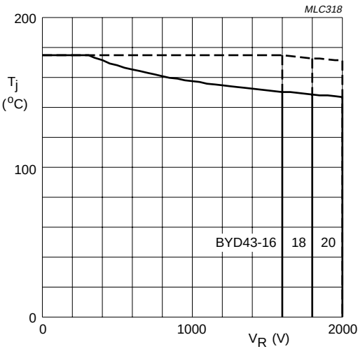
BYD43-16 to 20 Dotted line = V_{RRM} ; \delta = 0.1 . Solid line = V_{RRM} ; \delta = 0.5 .
