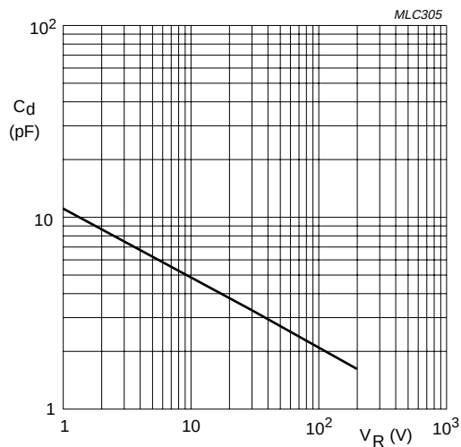
BYD43U and V f = 1 \text{ MHz}; T_j = 25 \text{ }^\circ\text{C}.
