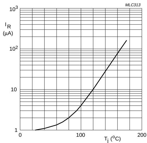
BYD43U and V V_R = V_{RRMmax} .
