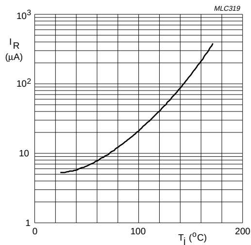
BYD43-16 to 20 V_R = V_{RRMmax} .
