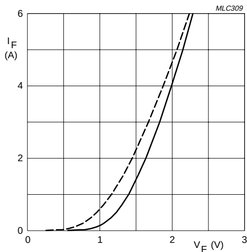
BYD43U and V Dotted line: T_j = 175\text{ }^{\circ}\text{C} . Solid line: T_j = 25\text{ }^{\circ}\text{C} .
