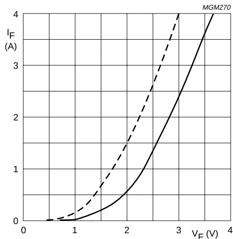
BYD57U and V Dotted line: T_j = 175\text{ °C} . Solid line: T_j = 25\text{ °C} .
