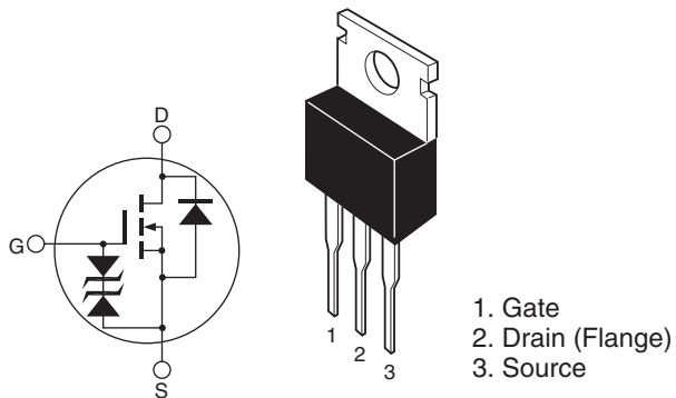
TO-220AB
