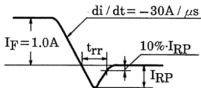
t_{rr} WAVEFORM
