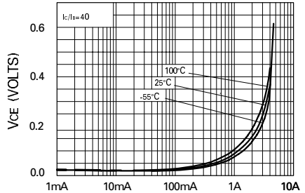
V_{CE(SAT)} vs I_C
