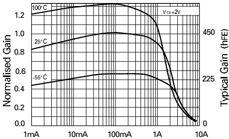
h_{FE} vs I_C
