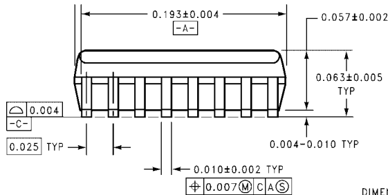
16-Lead Quarter Size Outline Package (QSOPT), JEDEC MO-137, 0.150 Wide Package Number MQA16
