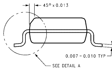
16-Lead Quarter Size Outline Package (QSOPT), JEDEC MO-137, 0.150 Wide Package Number MQA16
