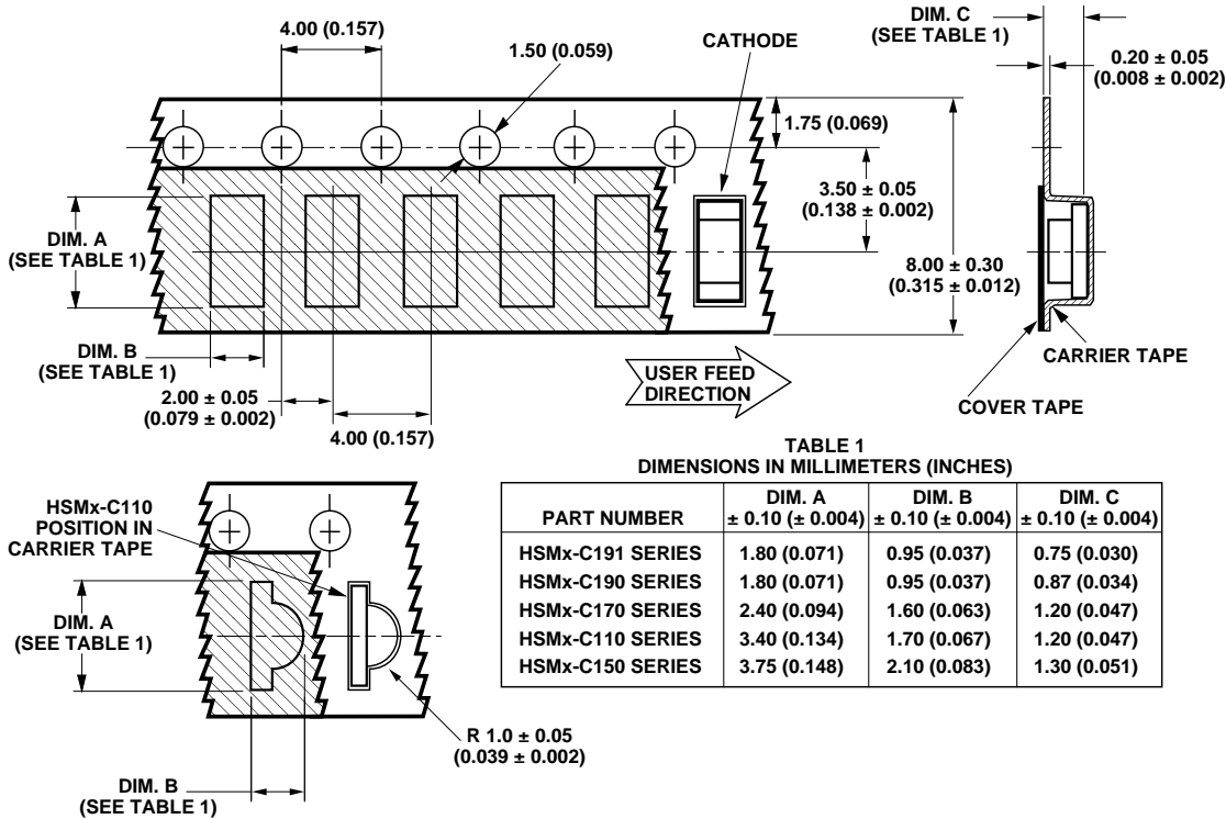
Figure 14. Tape Dimensions.
