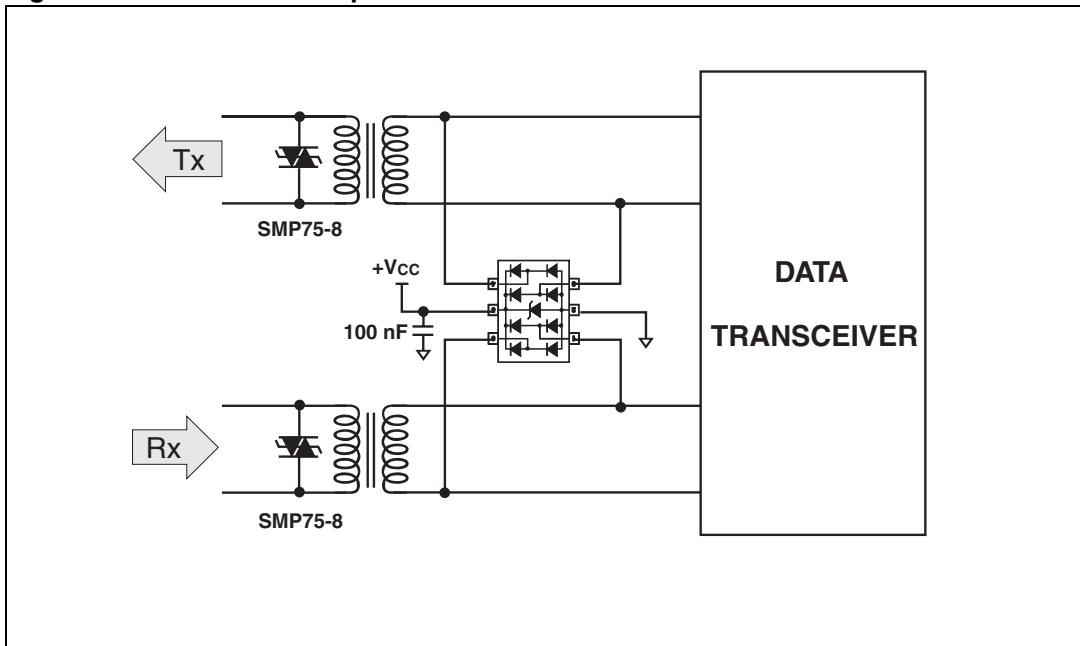
Figure 6. T1/E1/Ethernet protection
