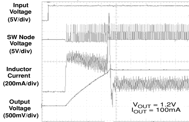
Start-up Response
