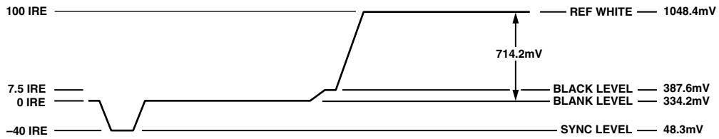
Figure 39. NTSC Luma Video Levels
