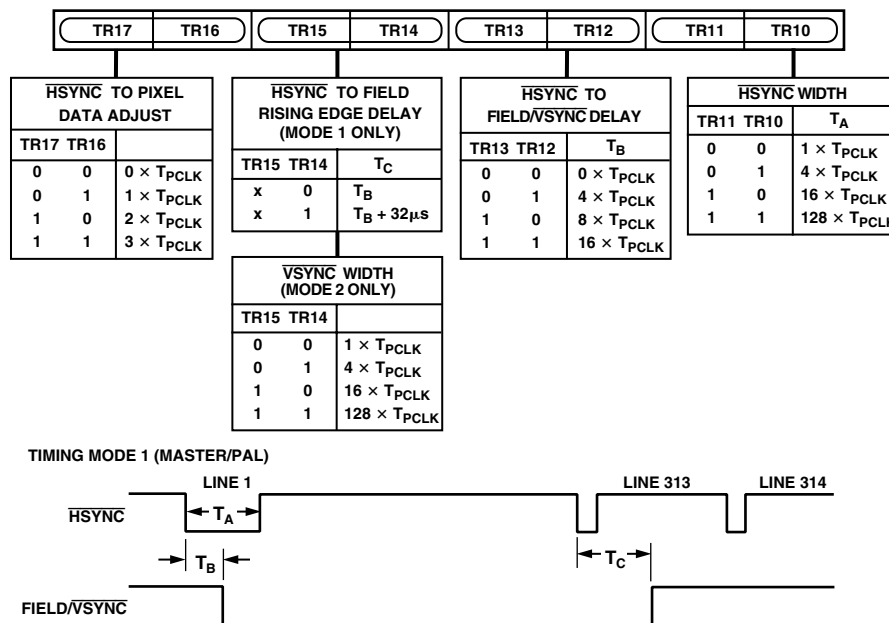
Figure 31. Timing Register 1
