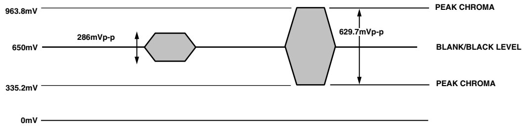
Figure 40. NTSC Chroma Video Levels
