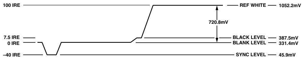
Figure 41. NTSC RGB Video Levels
