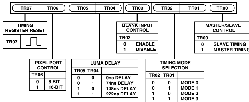
Figure 28. Timing Register 0
