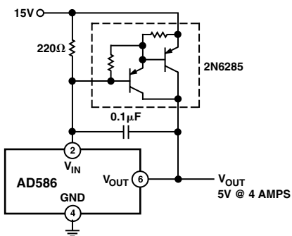
Figure 15b. Precision High-Current Voltage Source
