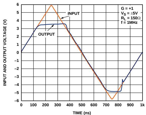
Figure 18. Input Overdrive Recovery
