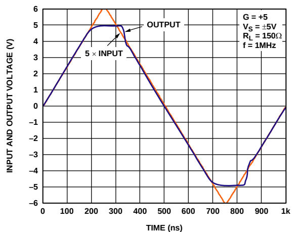
Figure 17. Output Overdrive Recovery
