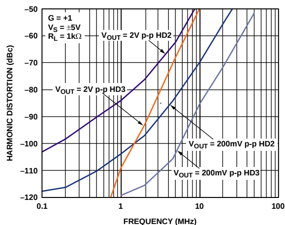
Figure 16. Harmonic Distortion vs. Frequency for Various V_{OUT}
