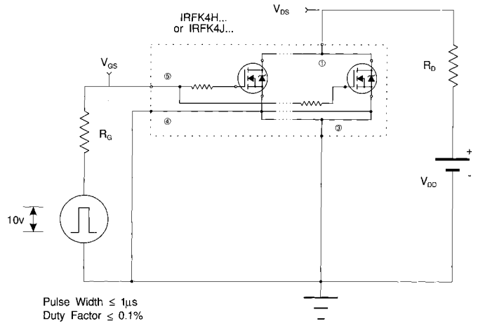
Fig 11a. Switching Time Test Circuit
