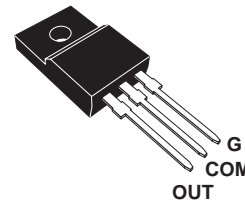
TO-220FPAB ACST4-7SFP/CFP
