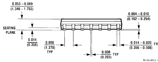
14-Lead Small Outline Molded Package (M) Order Number DM74LS09M NS Package Number M14A
