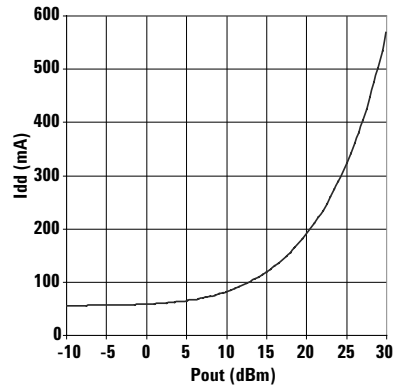
Figure 7. Total Idd vs Pout
