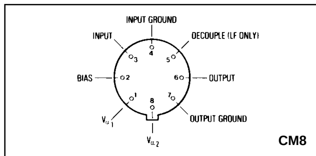
Fig.1 Pin connections
