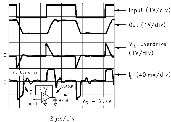
FIGURE 6. Buffer Amplifier Scope Photo
