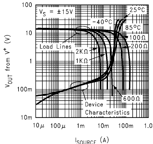
FIGURE 7. Output Sourcing Characteristics with Load Lines
