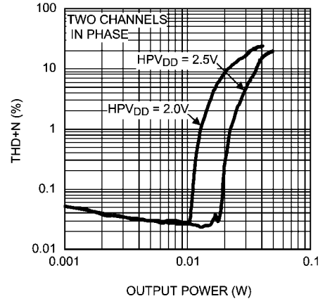
THD+N vs Output Power A_V = 0\text{dB} , R_L = 16\Omega , f = 1\text{kHz} Analog Input, Headphone Mode
