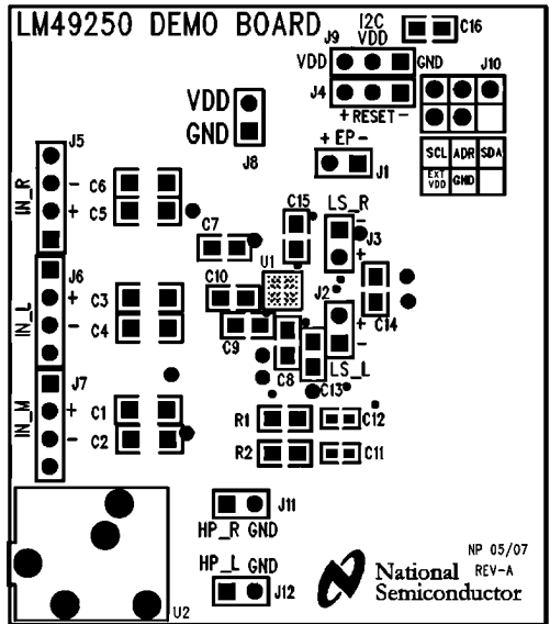
Top Silkscreen
