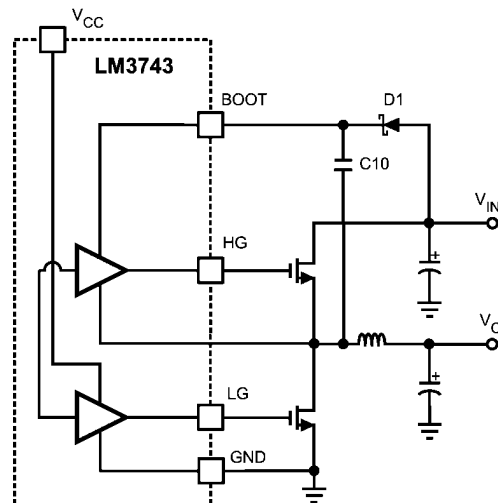
FIGURE 4. Charge Pump Circuit and Driver Circuitry
