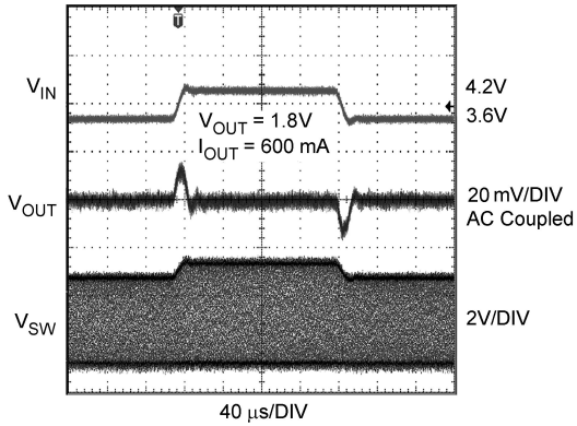
Line Transient Response V_{OUT} = 1.8V (PWM Mode)
