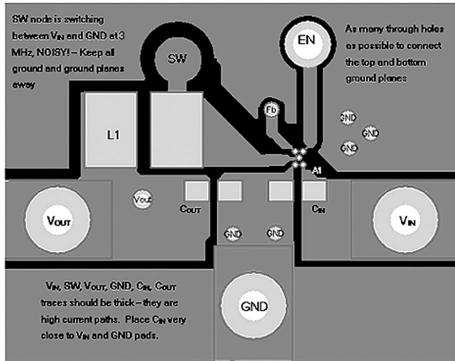
FIGURE 8. Board Layout Design Rules for the LM3677
