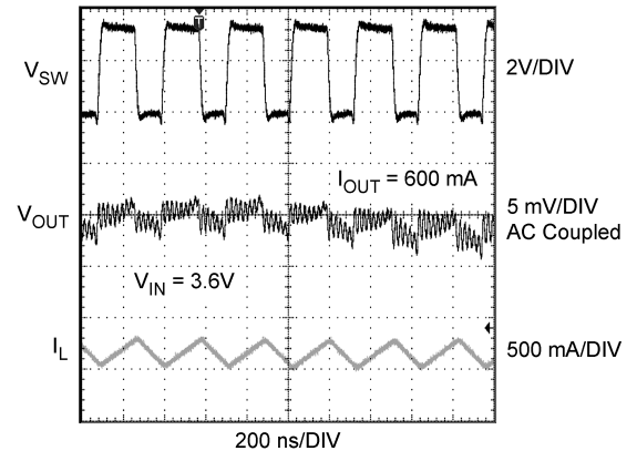
FIGURE 5. Typical PWM Operation
