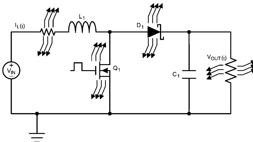
FIGURE 11. Thermal Schematic
