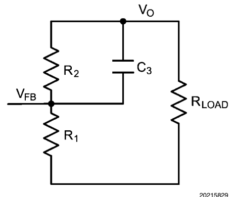
FIGURE 5. Setting Vout
