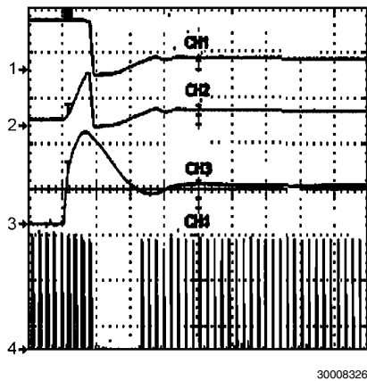
Vphase=10V CH1 = CO, 5V/Div CH2 = COMP, 5/Div CH3 = Iout, 10A/Div CH4 = SSPP Switch Signal, 4V/Div Horizontal Resolution= 20 \mu s/Div
